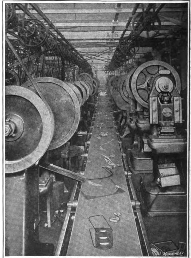
Fig. 34—In the Ford Motor Co.'s plant, use is made of belt conveyors for carrying away the product of power presses. Chutes are provided by means of which the product is transferred from the machines to the belt conveyor which carries it away. This is the means of saving the time ordinarily required for removing the product in trucks
